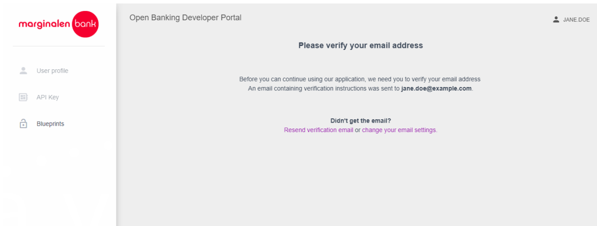
Figure 2 Email Verification
